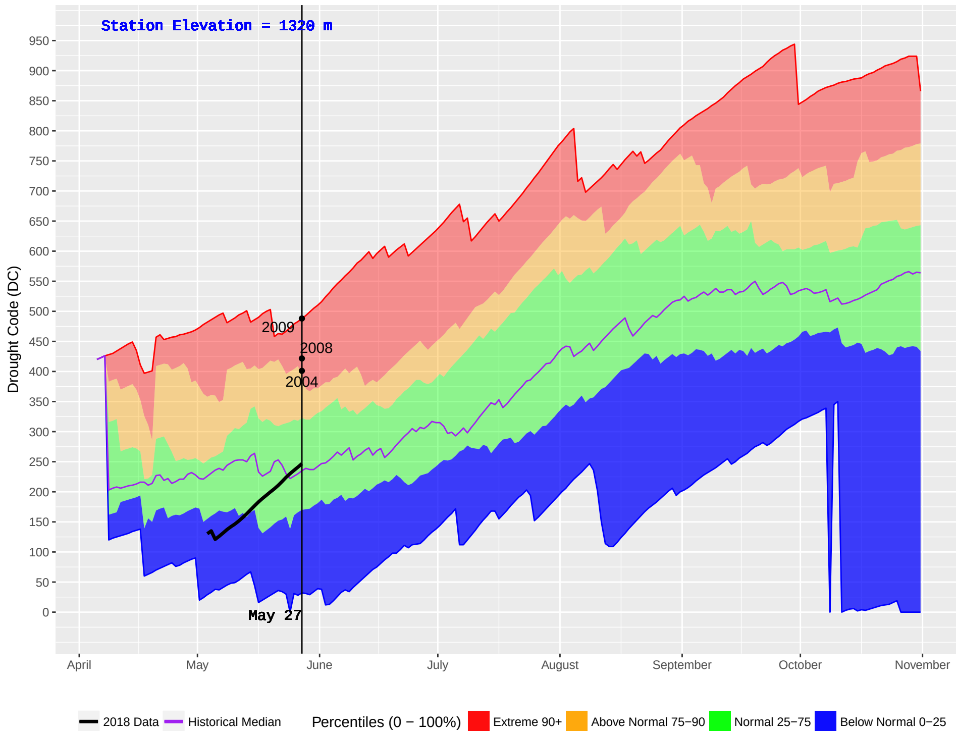
FRENCH BAR (306) : Historical (1979–2016) and Current (2018) Noon Drought Code (DC)
